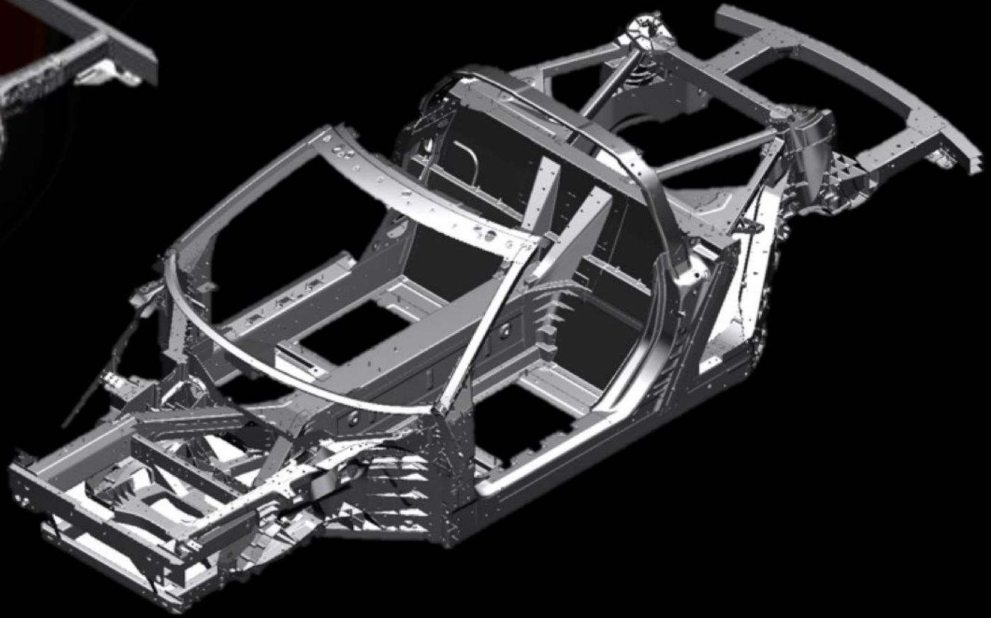
C8 Frame
